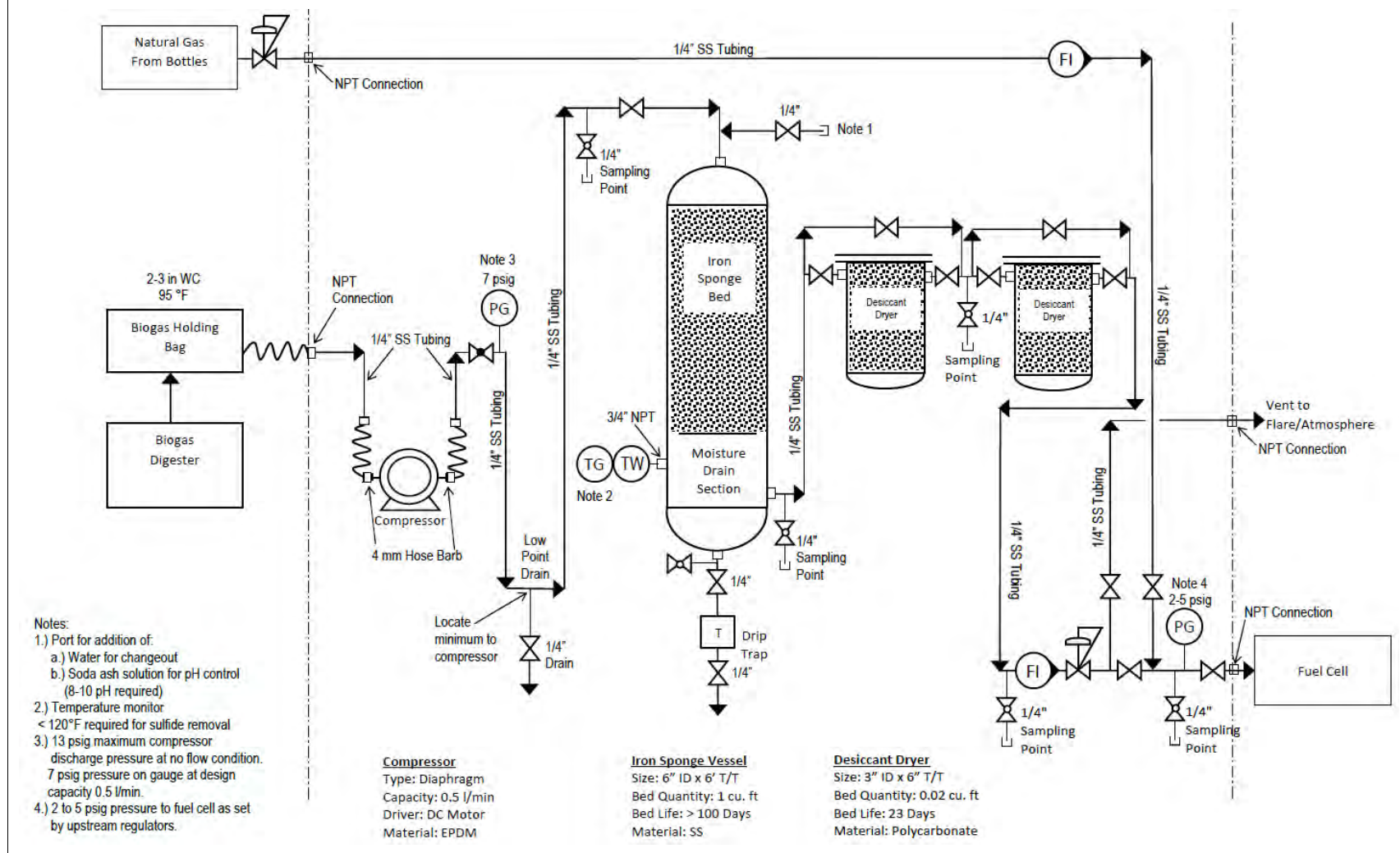
Figure 3-8 Biogas Conditioning and Compression Unit Piping and Instrumentation Diagram
