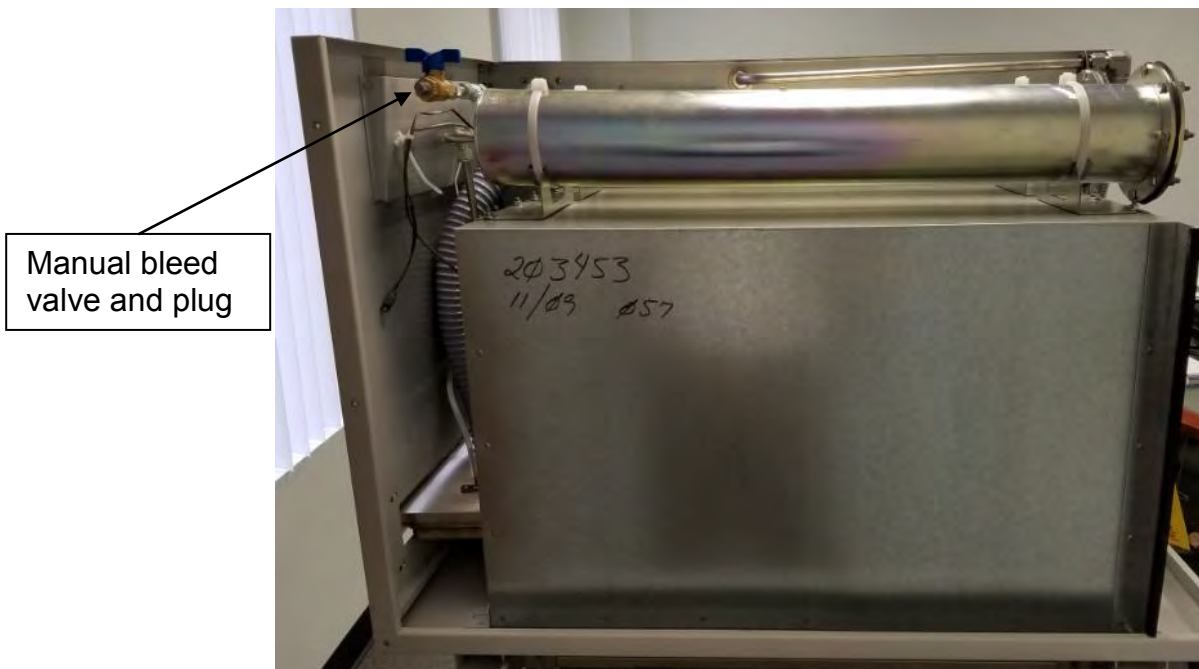
Figure 13: Manual Bleed Valve
