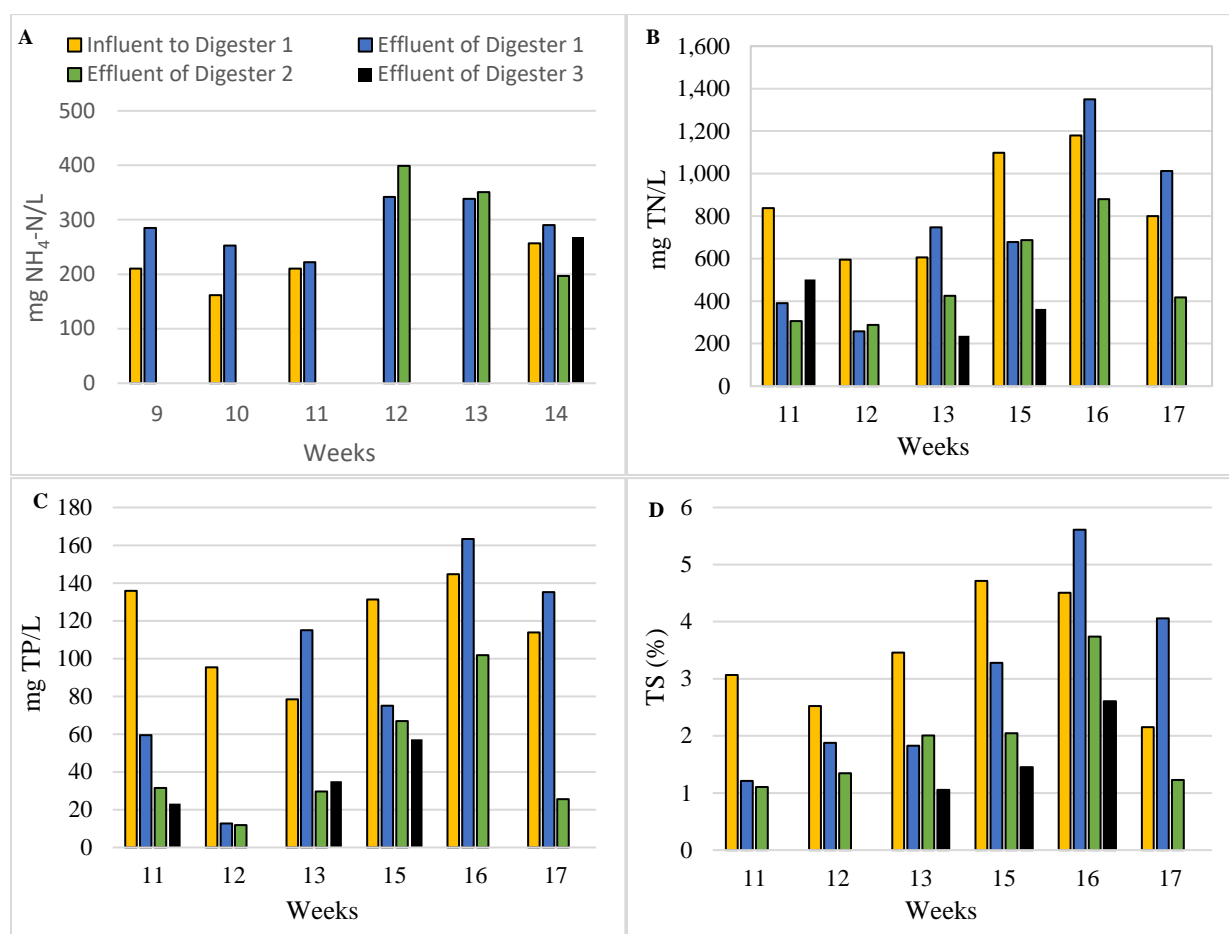
Figure B1-3: Nutrients and solids in the pilot-scale digestion system, with A) ammonium-nitrogen ( \text{NH}_4\text{-N} ) concentrations, B) total nitrogen (TN) concentration, C) total phosphorus (TP) concentrations, and D) percent total solids (TS).
