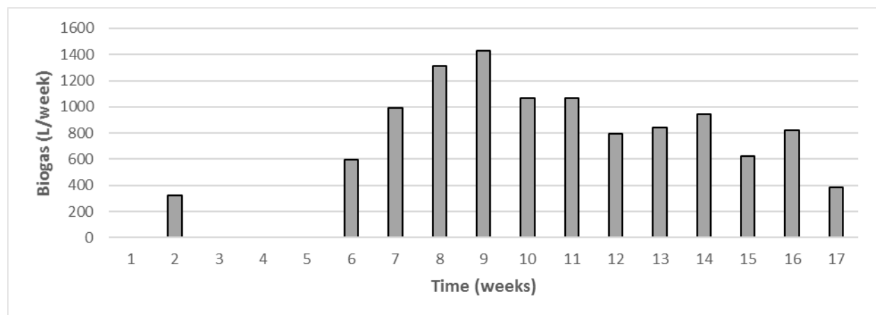
Figure 4-7 Total Weekly Biogas Production
