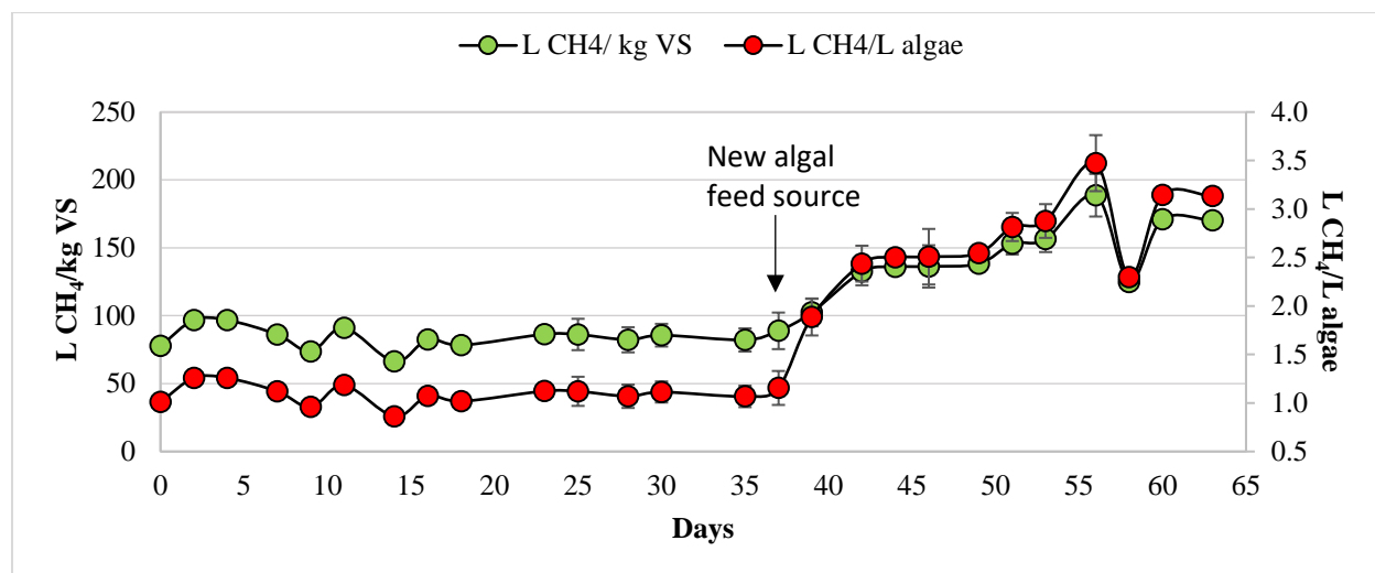
Figure B2-2: Methane ( \text{CH}_4 ) production per kg volatile solids (VS) and per liter of algae for the continuous reactors during the 64-day testing period.
