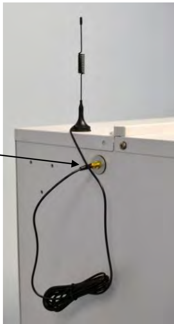
Figure 8: Antennae connection
