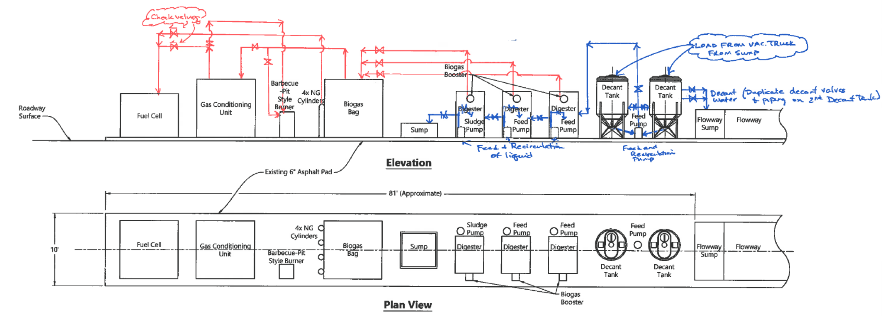
Figure 3-4 System Piping
